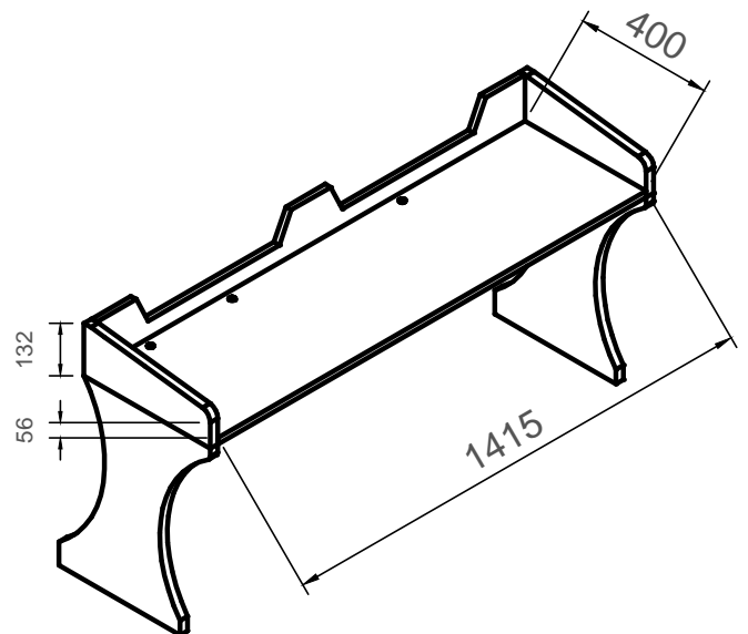
KEYBOARD TRAY
