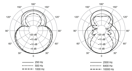
Polar Patterns
