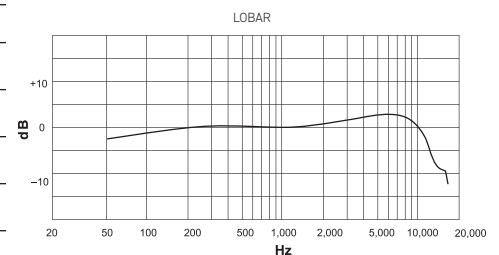
Frequency Response
