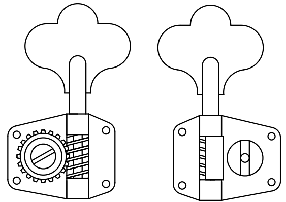
rechte Mechanik right machine head
