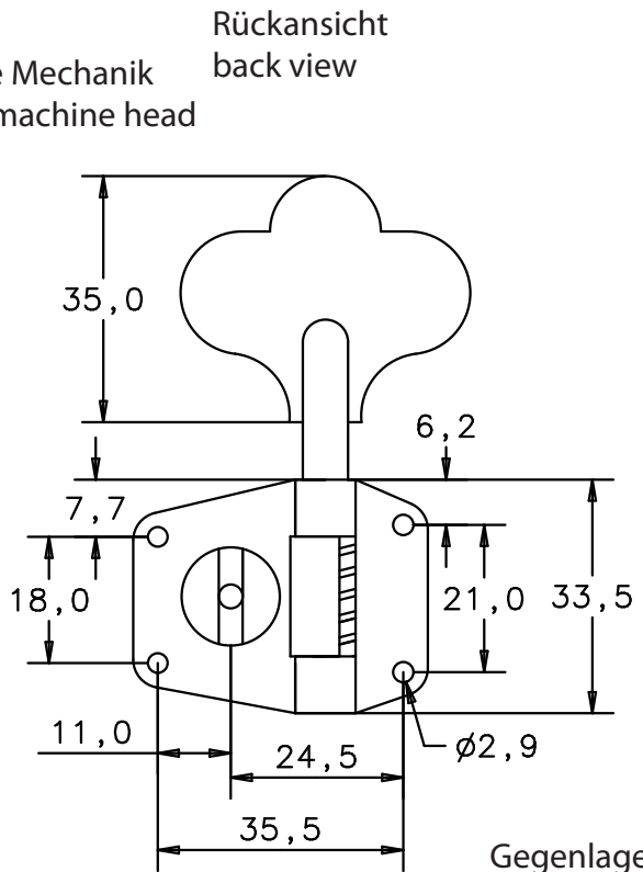
rechte Mechanik right machine head
